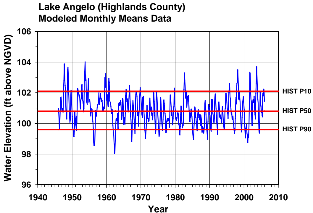
Figure 5. Modeled monthly-means surface water elevations in feet above NGVD 29 for the composite data set from January 1946 through December 2005 for Lake Angelo, and the Historic P10, P50, and P90 lake stage percentile elevations.
