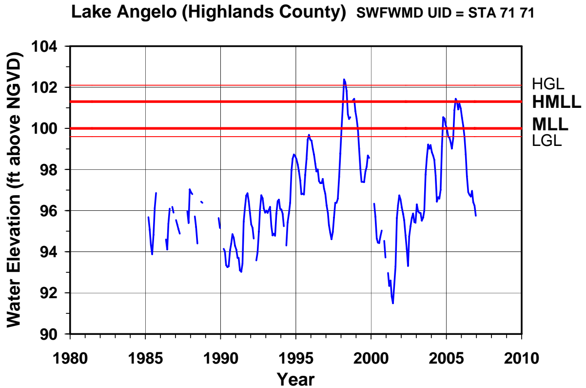
Figure 7. Mean monthly surface water elevations in feet above NGVD 29 through December 2006 based on measured lake stage records, and Minimum and Guidance Levels for Lake Angelo. Levels include the High Guidance Level (HGL), Low Guidance Level (LGL), High Minimum Lake Level (HMLL), and Minimum Lake Level (MLL).
