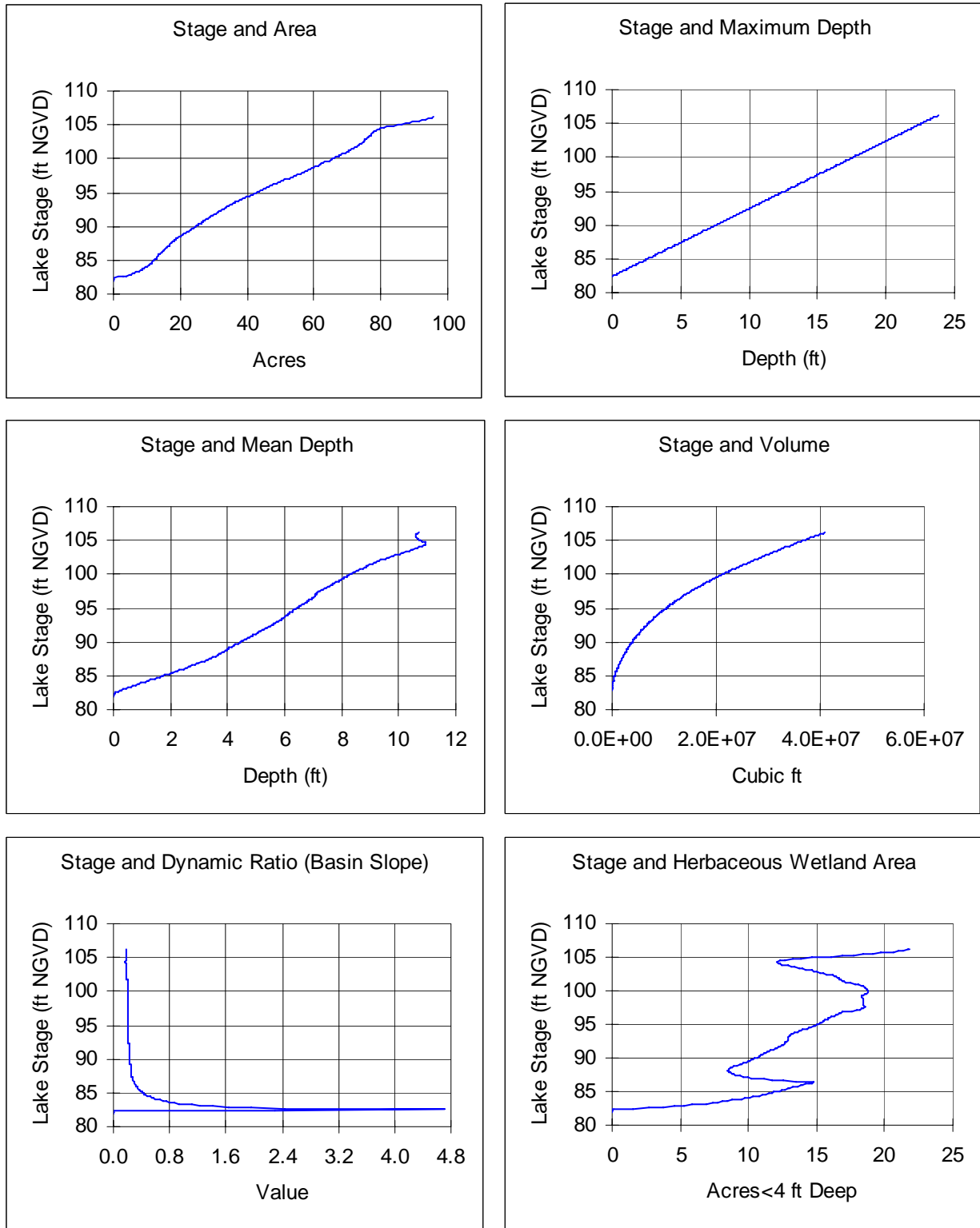
Figure 6. Surface area, maximum depth, mean depth, volume, dynamic ratio (basin slope), and potential herbaceous wetland area versus lake stage in feet above NGVD 29 for Lake Angelo.
