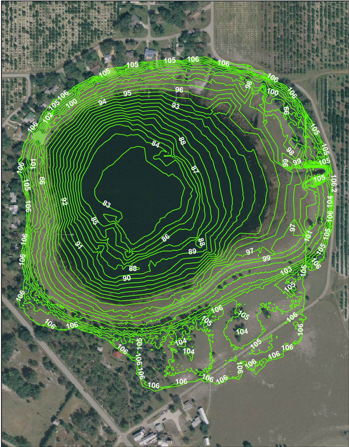
Figure 3. One-foot contours within the Lake Angelo basin. Values shown are elevations in feet above NGVD 29.
